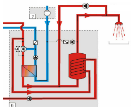
Fig. 1: Fresh water unit for large solar thermal systems. Source: Solvis.
