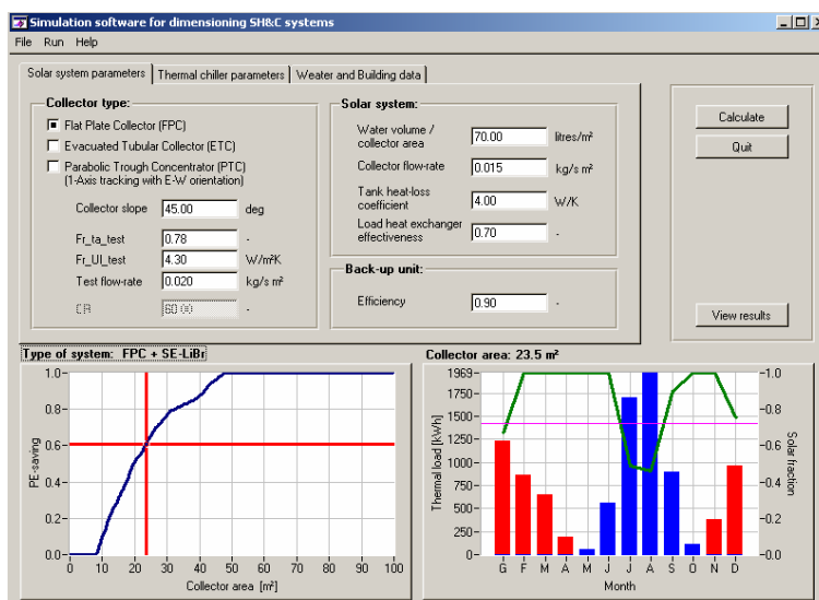
Fig. 3: Graphical user interface of the solar cooling design tool
