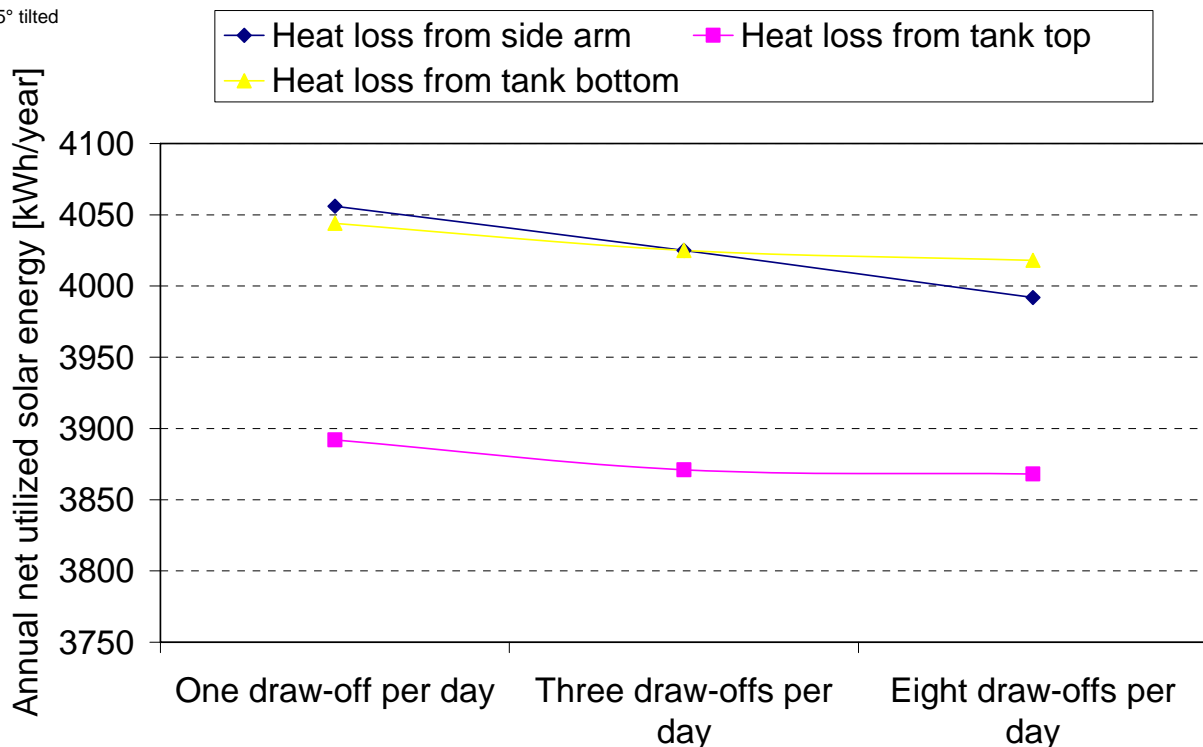
Figure 4. Yearly net utilized solar energy for a solar heating system with different distributions of the heat loss coefficient.
